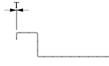
SECTION VIEW Y-Y SCALE (1 : 4) VIEW ROTATED AND ENLARGED PROFILE MIRRORED OPP SIDE
