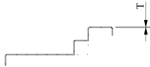
SECTION VIEW Z-Z SCALE (1 : 4) VIEW MIRRORED OPP SIDE
