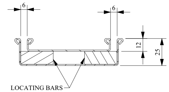
SECTION VIEW A-A SCALE (1 : 2)
