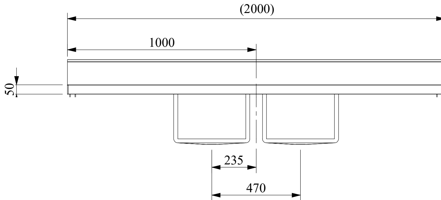
Benchtop and bowl elevation
